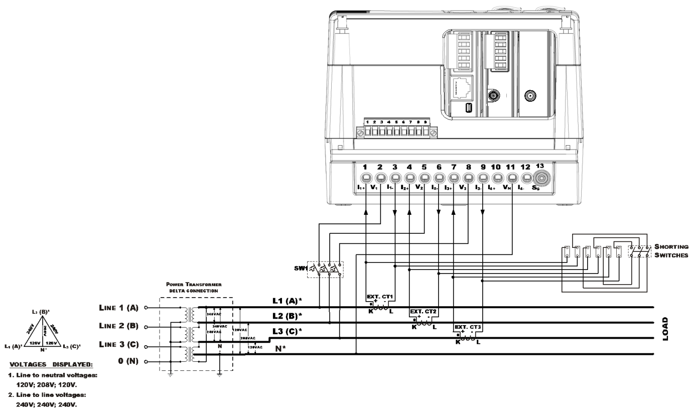
Figure 12: Four Wire Delta Connection Using 3 CTs - Wiring Setup: 4LL3 or 4Ln3
