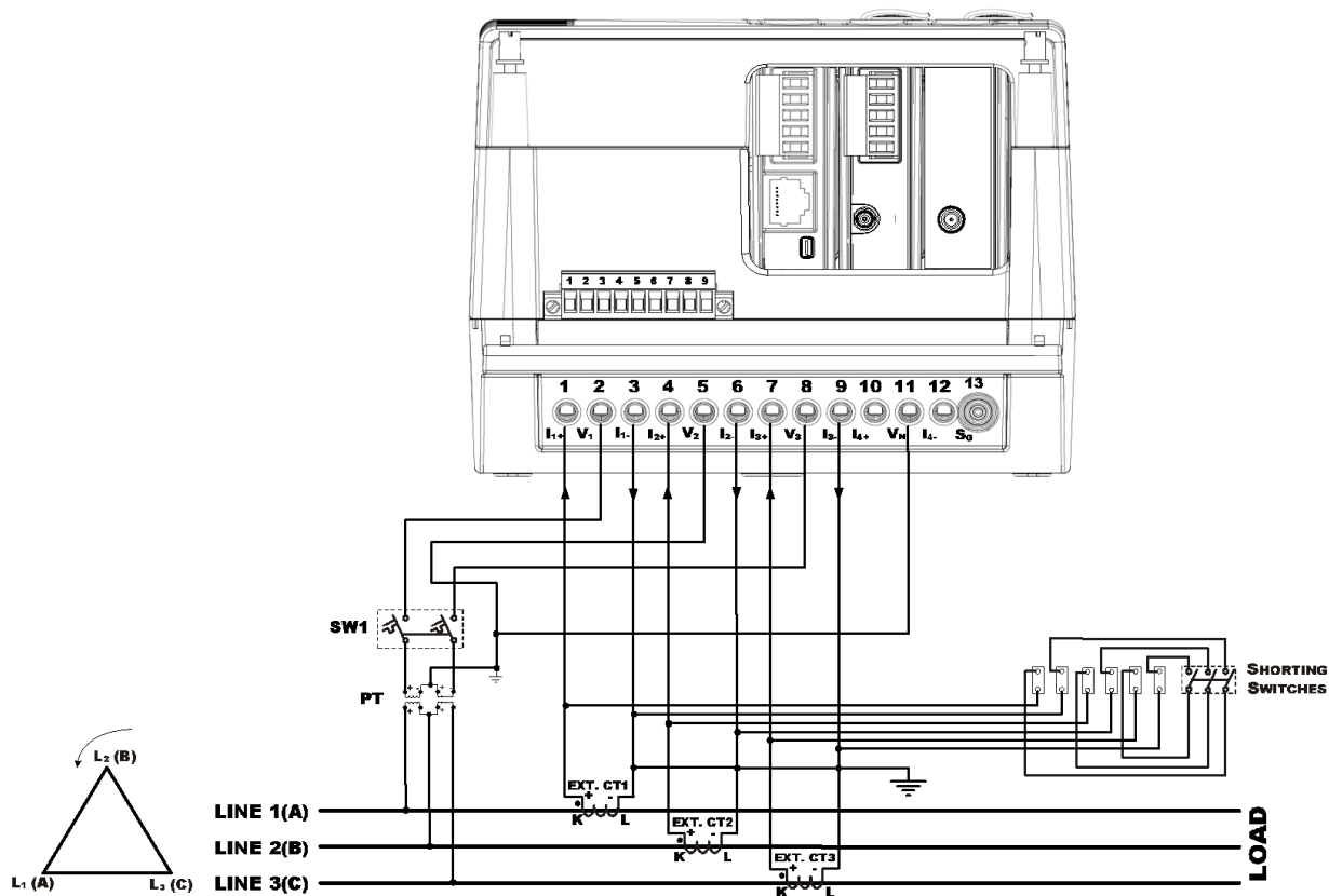
Figure 11: Three Wire Open Delta Connection Using 2 PTs, 3 CTs - Wiring Setup: 3OP3 Energy is measured with 2 CTs only - Phases 1(A) and 3(C)
