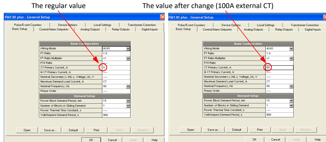
Figure 4: In device General Setup (PAS Software) “CT Primary Current” should be modified with the nominal value of the used CT (the illustrated case is I_n=50A for 100A external CT).
