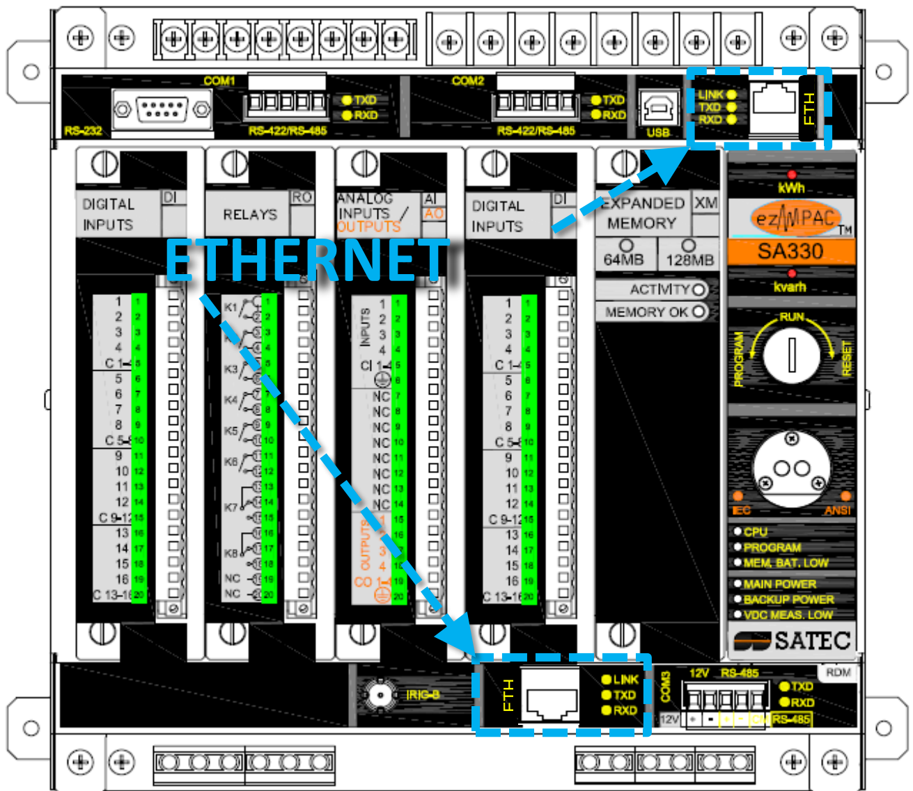
Figure 1: Dual Ethernet Port ezPAC top view.
