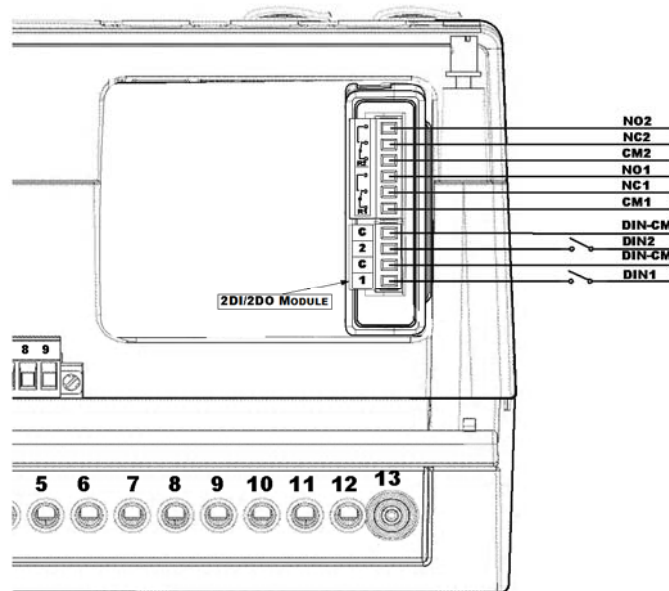
Figure 14: 2DI/2DO Connection
